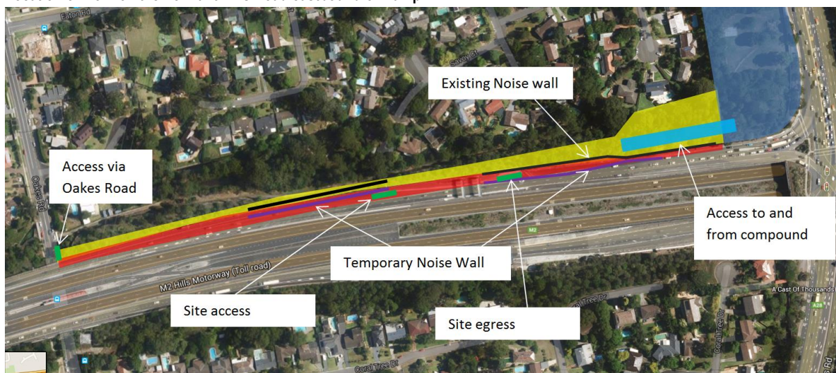
Location of work on the Pennant Hills Road eastbound off-ramp
